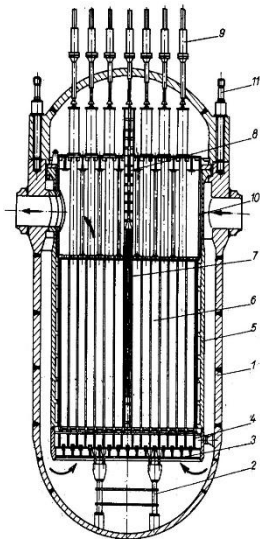
Figure 6.3: Pressurised water reactor (PWR) – Biblis nuclear power plant.
