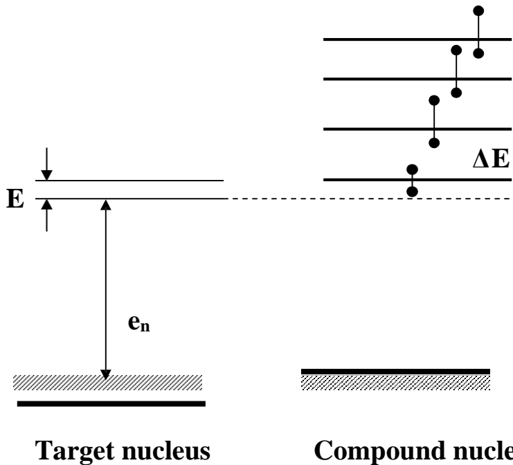
Figure 5.4: Energy levels of a compound nucleus.
