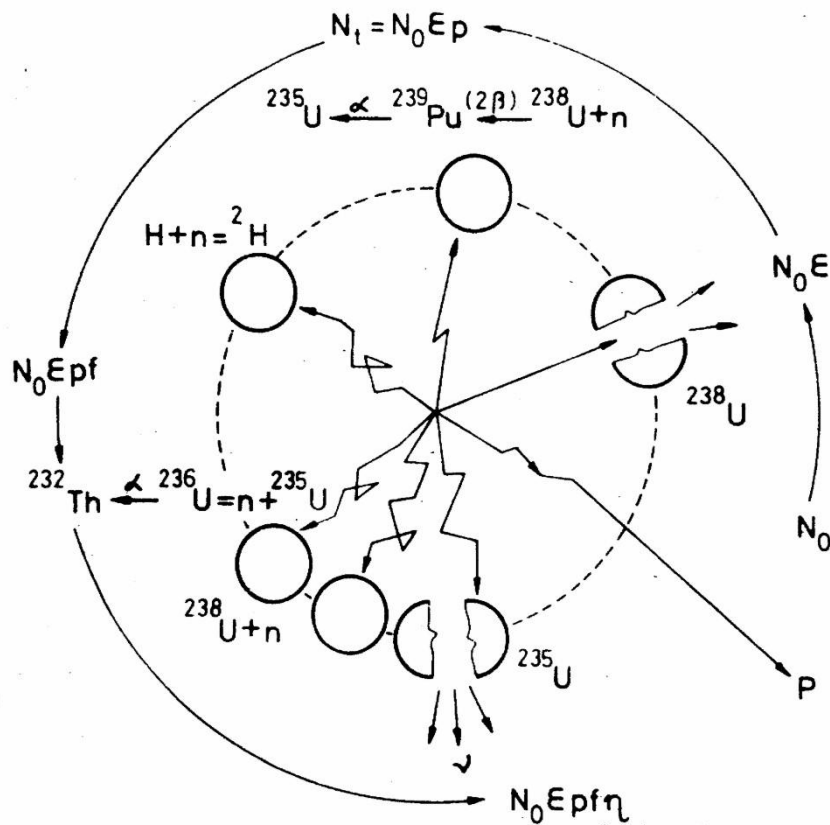
Figure 5.5: Neutron balance in the reactor core.
