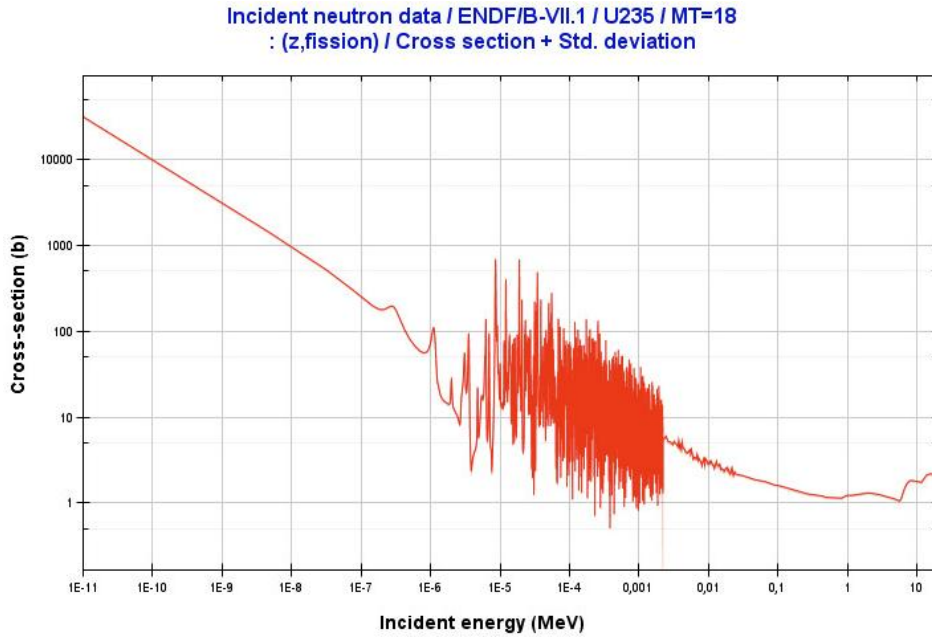
Figure 5.3 Energy-dependent microscopic cross-section of the absorption.
