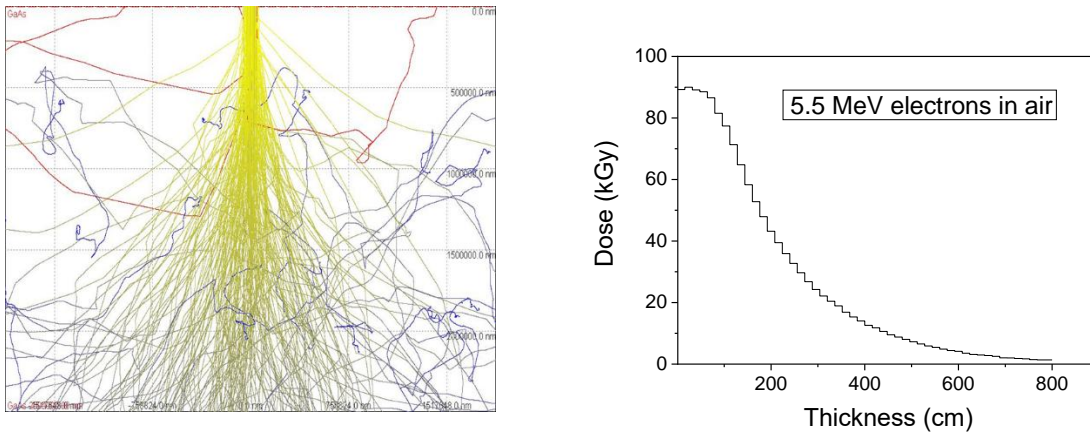
Figure 3.2: CASINO simulated trajectories of light charged particles (5 MeV \beta -particles) in GaAs (left). Energy deposition by 5.5 MeV \beta -particles as a function of penetration depth in the air, with long (> 6 m), more gradual decrease, simulation in ModePEB (right).
